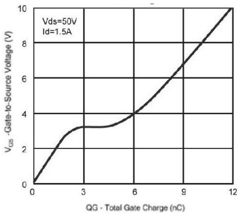
Figure 5: Gate-Charge Characteristics
