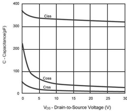
Figure 3: Capacitance
