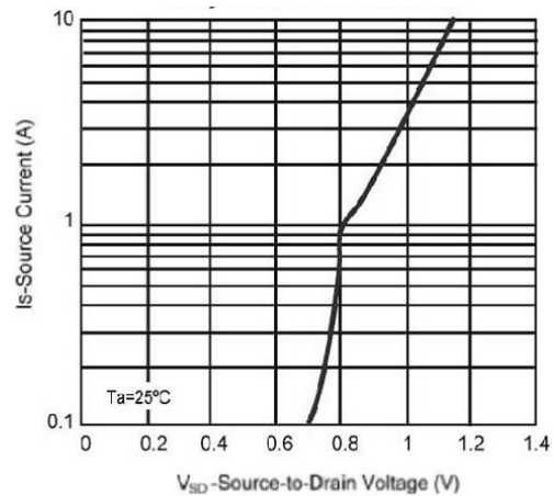
Figure 6: Body Diode Characteristics
