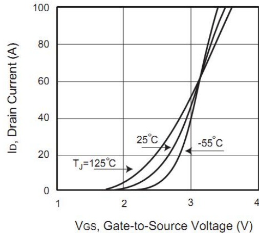
V_{GS} , Gate-to-Source Voltage (V) Figure 4. Transfer Characteristics
