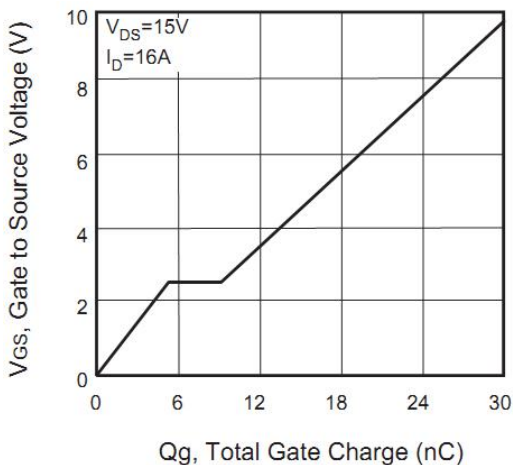
Q_g , Total Gate Charge (nC) Figure 5. Gate charge VS. Gate-source Voltage
