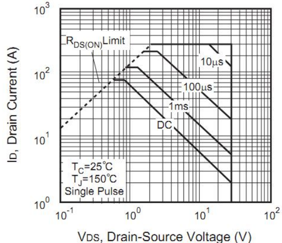
V_{DS} , Drain-Source Voltage (V) Figure 6. Maximum Safe Operating Area
