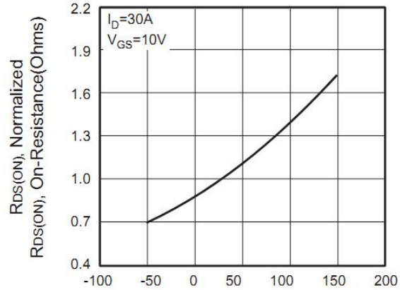
T_J , Junction Temperature ( ^{\circ}C ) Figure 2. On-Resistance Variation with Temperature
