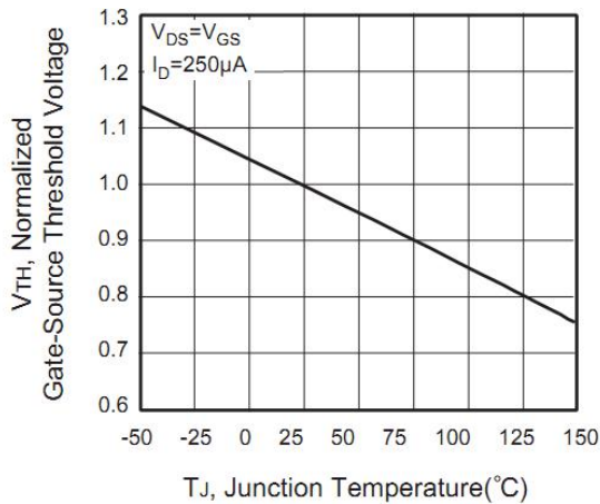
T_J , Junction Temperature ( ^{\circ}C ) Figure 3. Gate Threshold Variation with Temperatures
