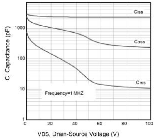
Figure 4: Capacitance Characteristics
